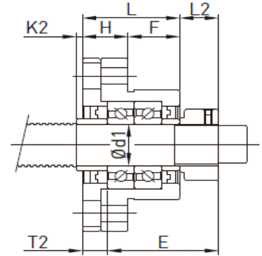
Mounting method B
