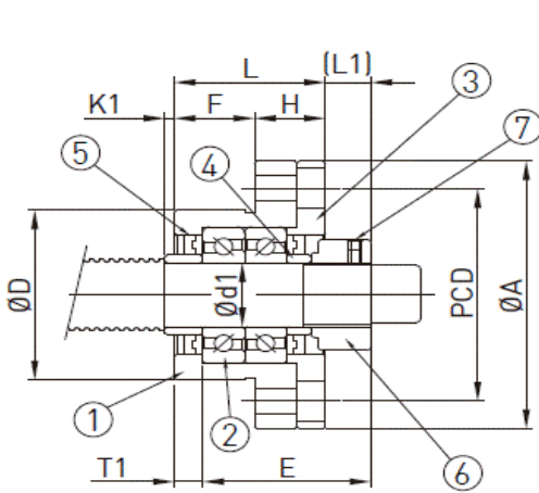
Mounting method A
